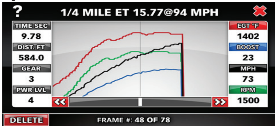
Figure 21 Performance Test Results
