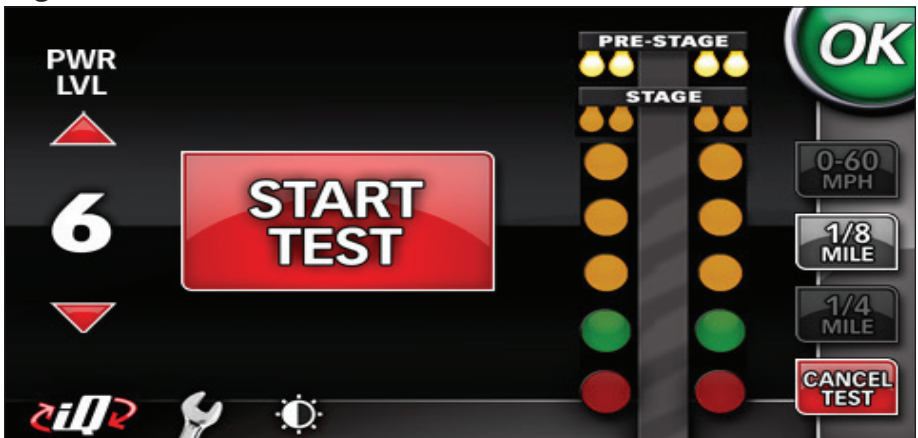
Figure 20 Start Test
