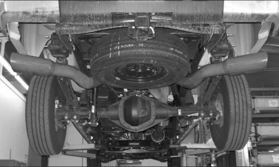
Figure 48 Split-Dual Exhaust
