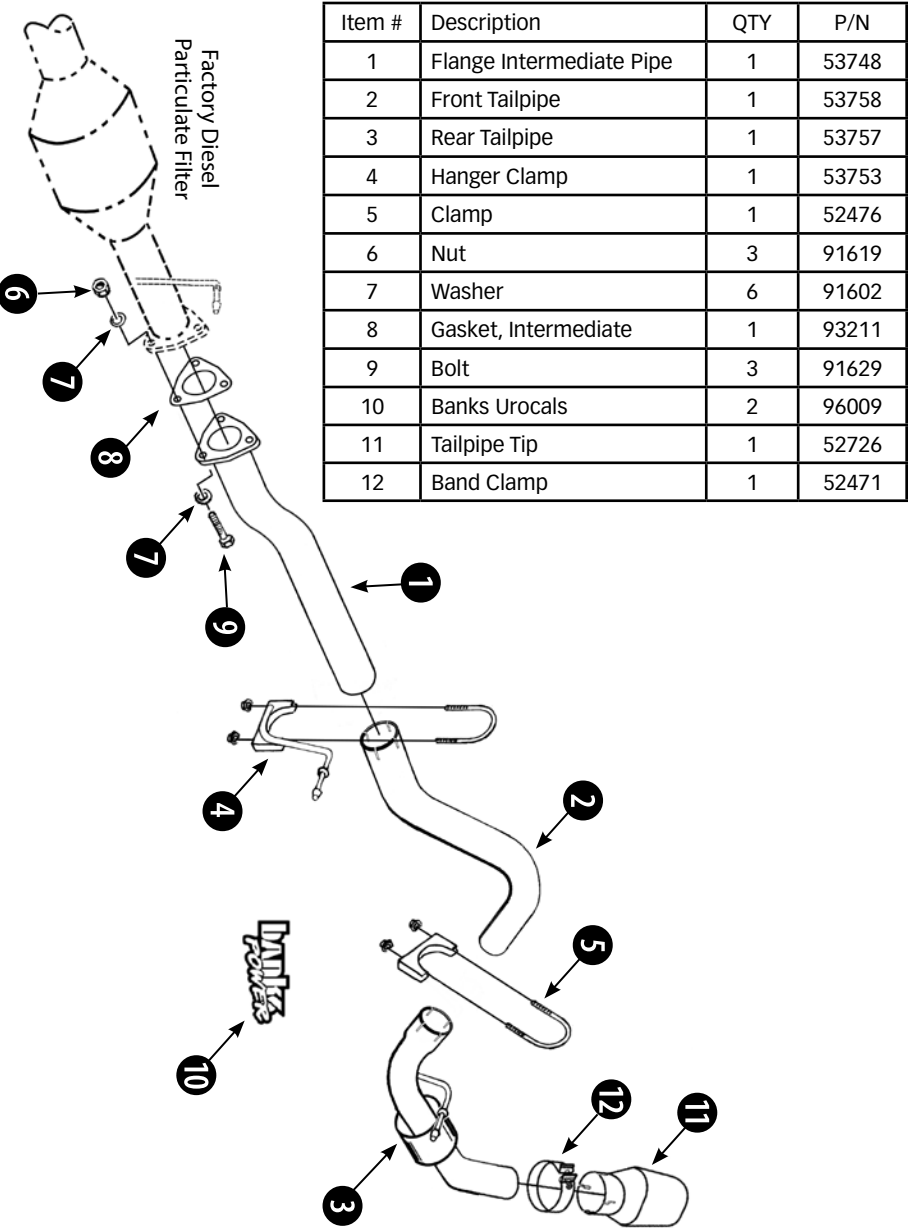
Figure 39 Banks Monster Exhaust, General Assembly
