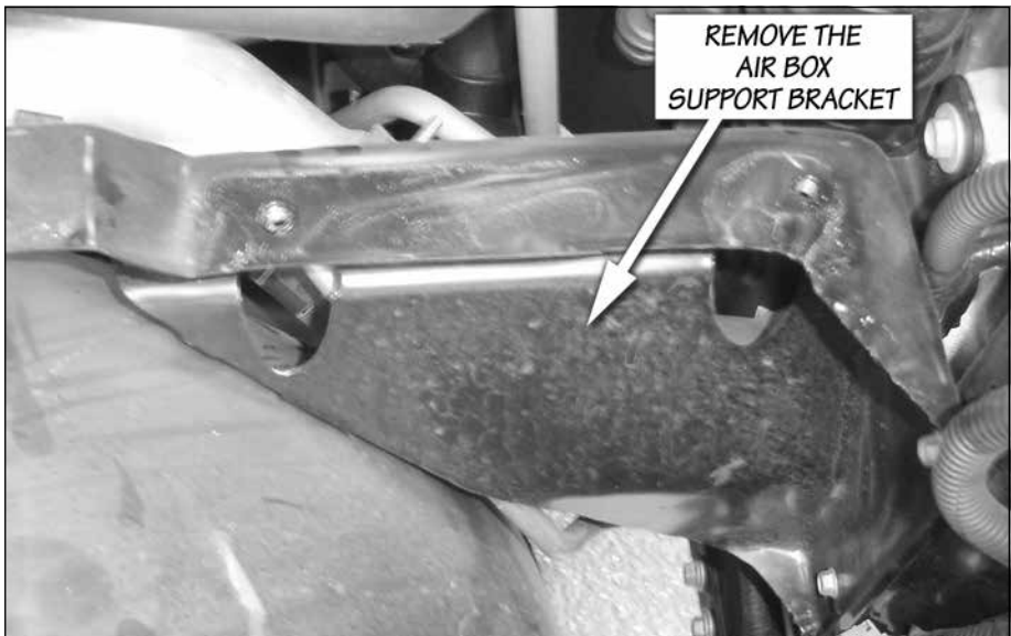
Figure 15 Air box support bracket
