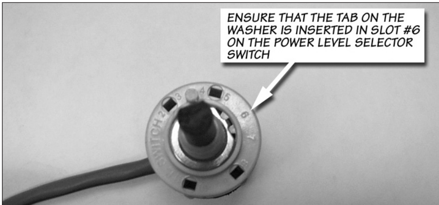
Figure 49: Finished installation of the Power Level Selector Switch on 2003-04 model year vehicles
