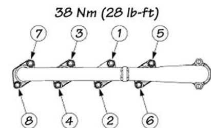
Figure 25: Exhaust manifold tightening sequence
