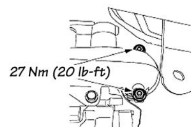
Figure 26: Turbocharger adapter pipe torque specification
