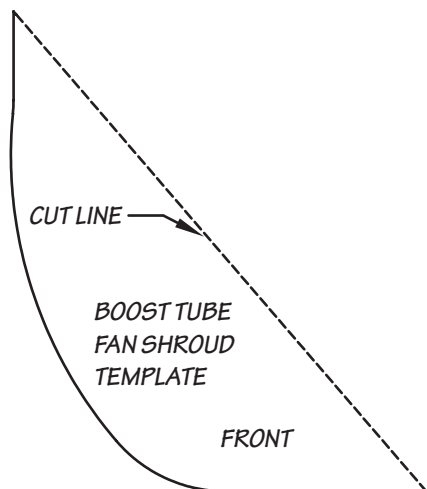
Template 1 (fan shroud, step 34)
