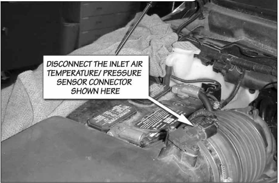
Figure 1 Location of the Inlet Air Temp/Pressure Sensor
