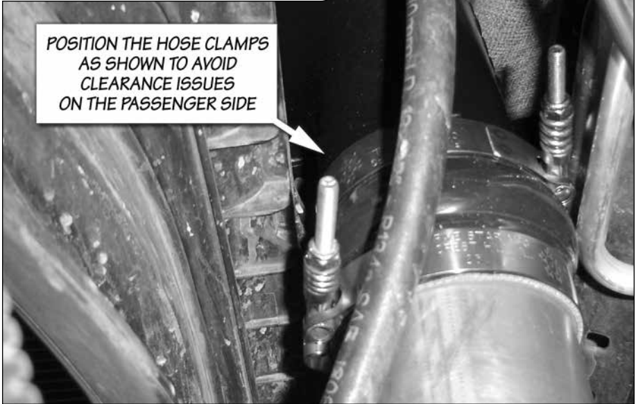
Figure 7 Orientation of the Passenger Side Hose Clamps to avoid clearance issues.
