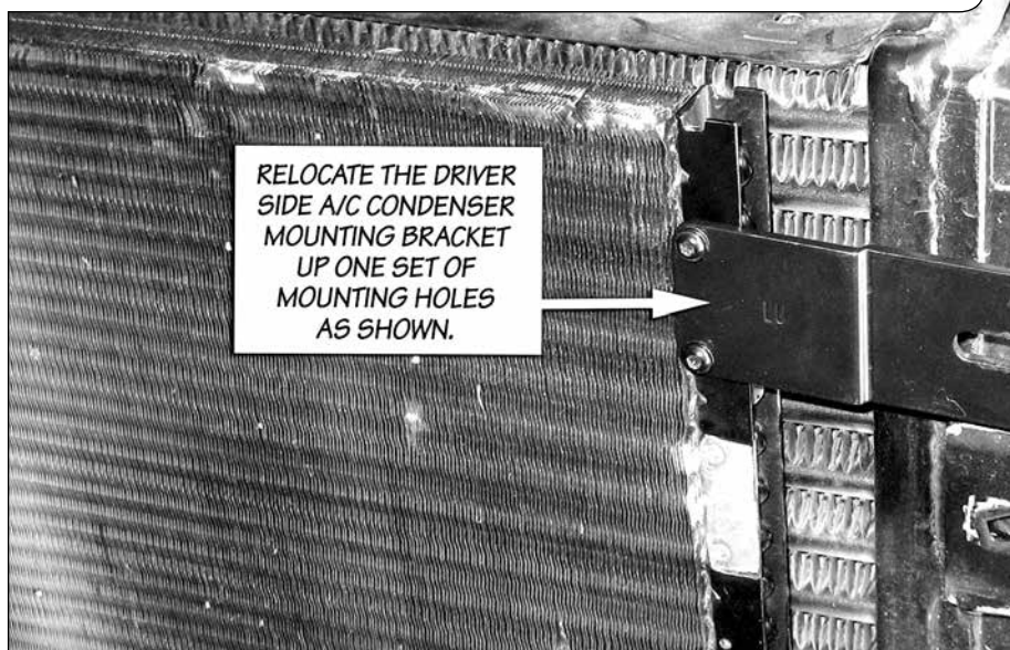
Figure 4 Relocation of the Upper Driver Side A/C Condenser Mounting Bracket
