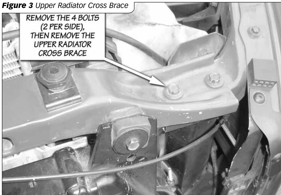
Figure 3 Upper Radiator Cross Brace
