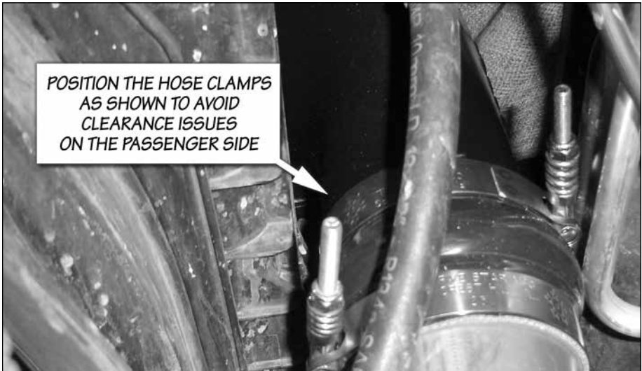
Figure 7 Orientation of the Passenger Side Hose Clamps to avoid clearance issues.
